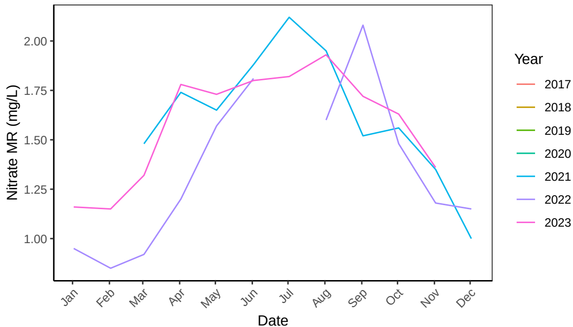
B2 Raceway 2 Nitrate MR (mg/L) Monthly Statistics
